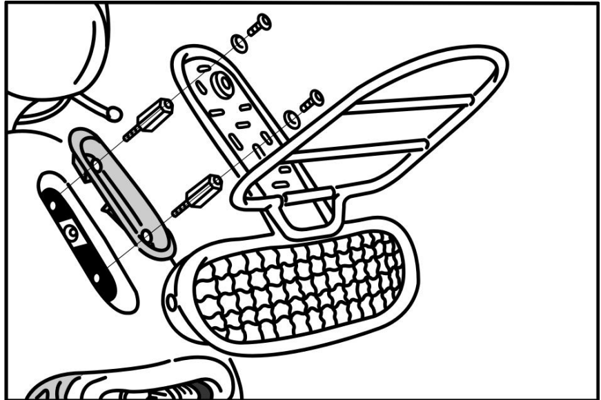
OFF-ROAD FRONT RACK - 2
